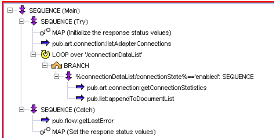
The underlying implementation of the web service under test.
