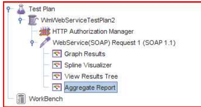
A sample JMeter test plan.
