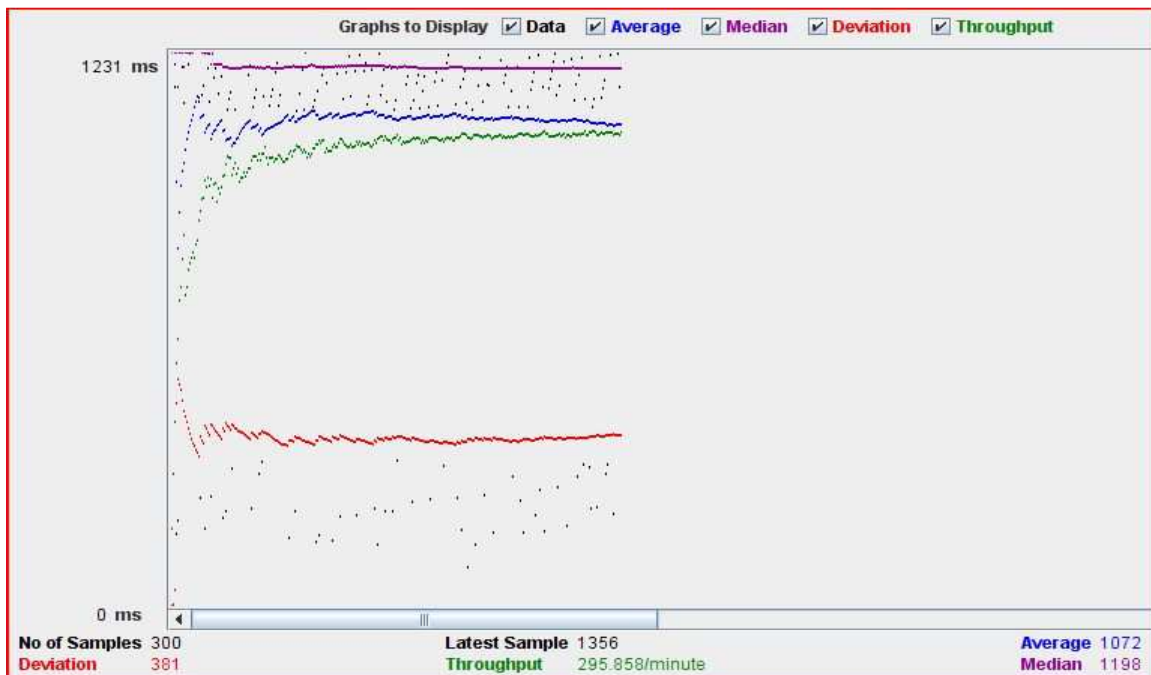
The Graph Result for the selected ThreadGroup configuration.
