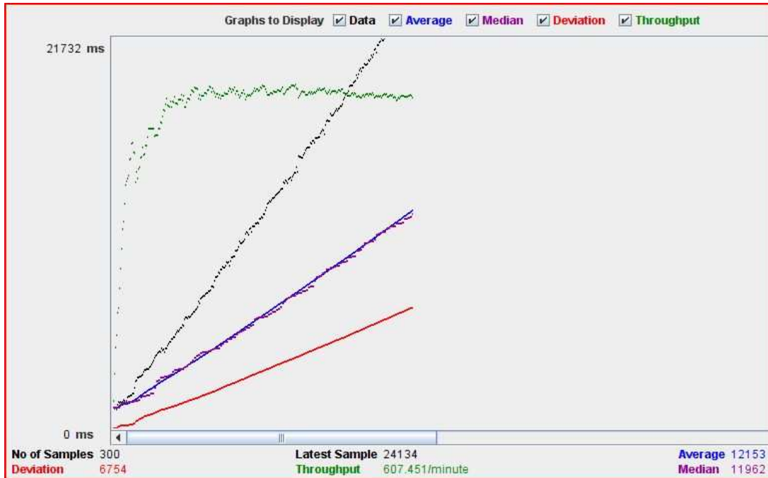
The Graph Result for the selected ThreadGroup configuration.
